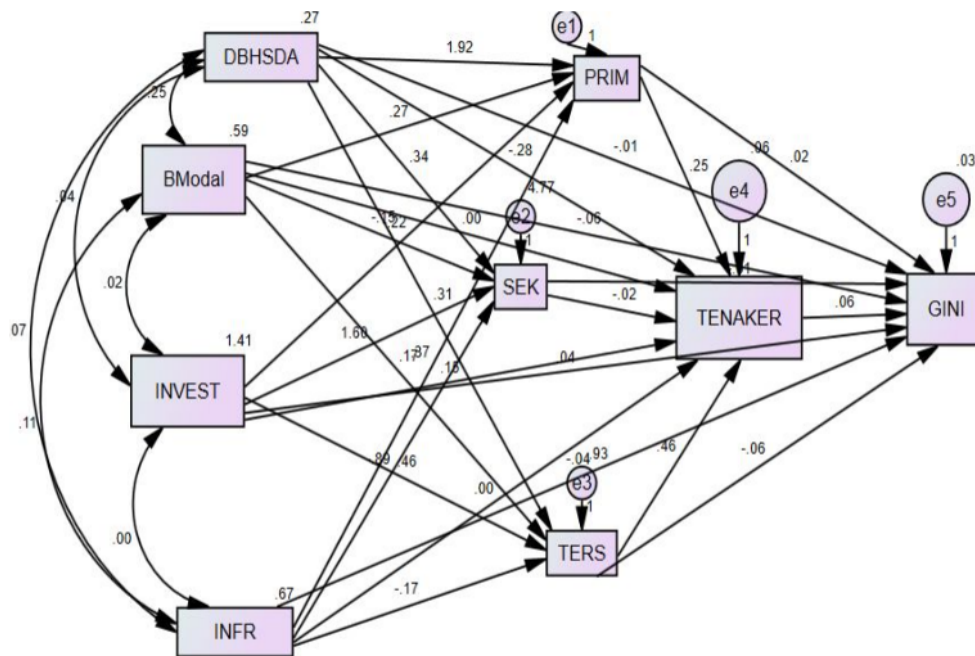
Figure 3. Path Structural Model Diagram (Unstandardized Coefficient)
