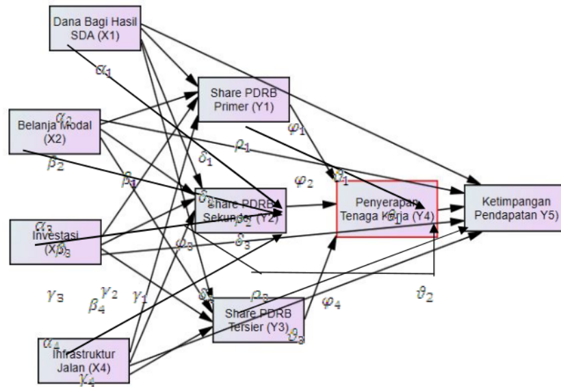
Figure 2. Path Schematic Structural Model
